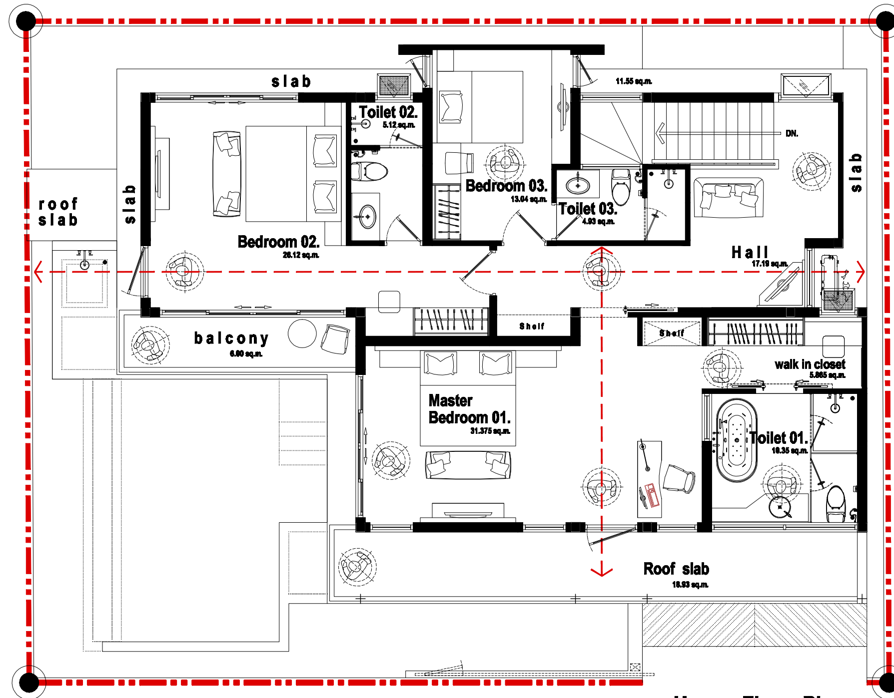
Upper Floor Plan scale 1:75
